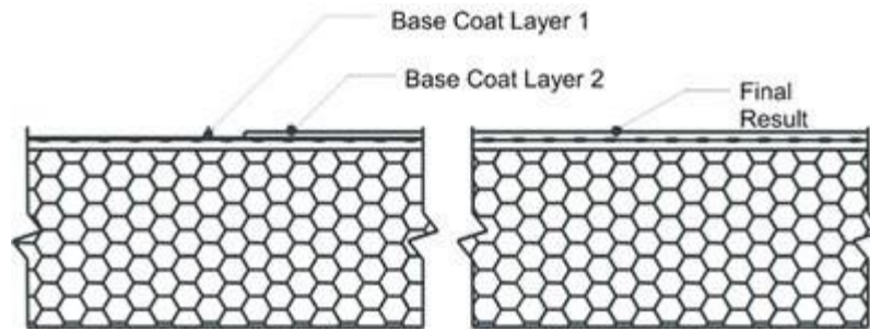
Fig. 11: Reinforcing Mesh
