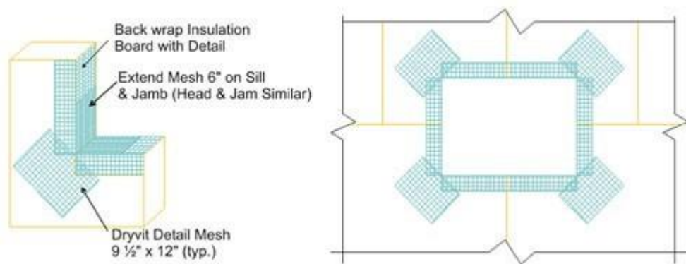
Fig. 10: Rough Openings
