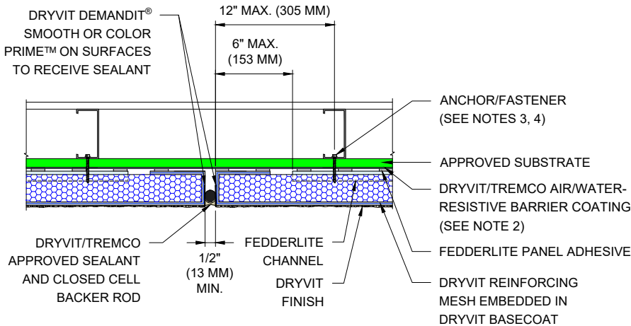
SECTION A
